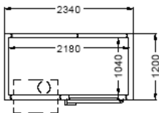
CRM/FRM 2340x1200 mm
